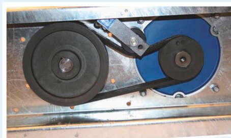
Transmission Mobile auger 152. Automatic tension of the poly V-belt.
