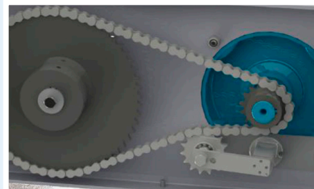
Transmission Mobile auger 200. Automatic tension of the chain.
